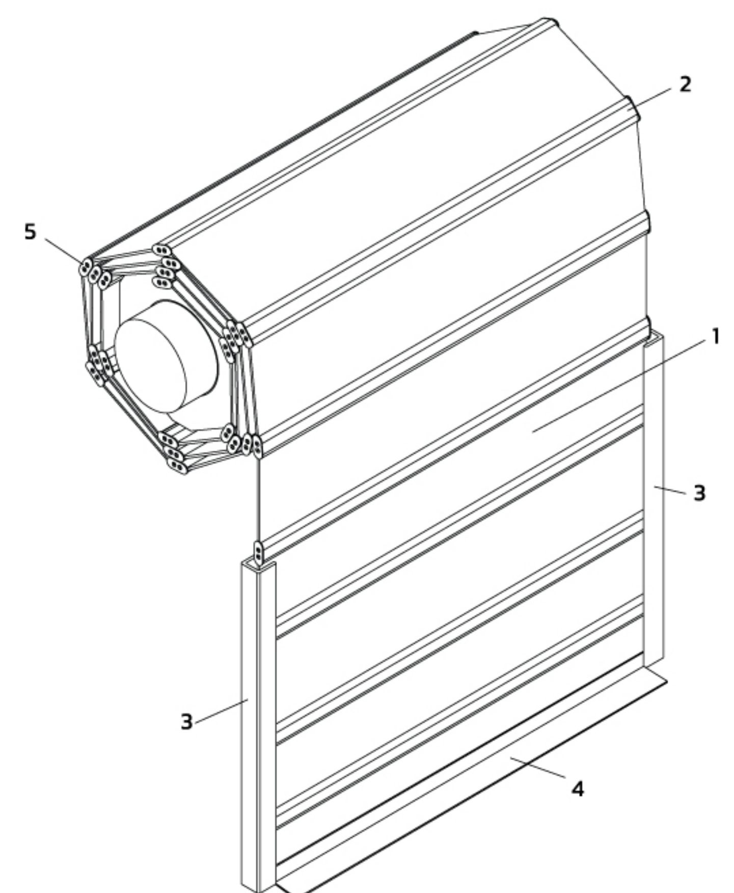
1.Polycarbonate sheet 2.Profile connector 3.Guide rail 4.Bottom bar 5.Stainless steel side cap
